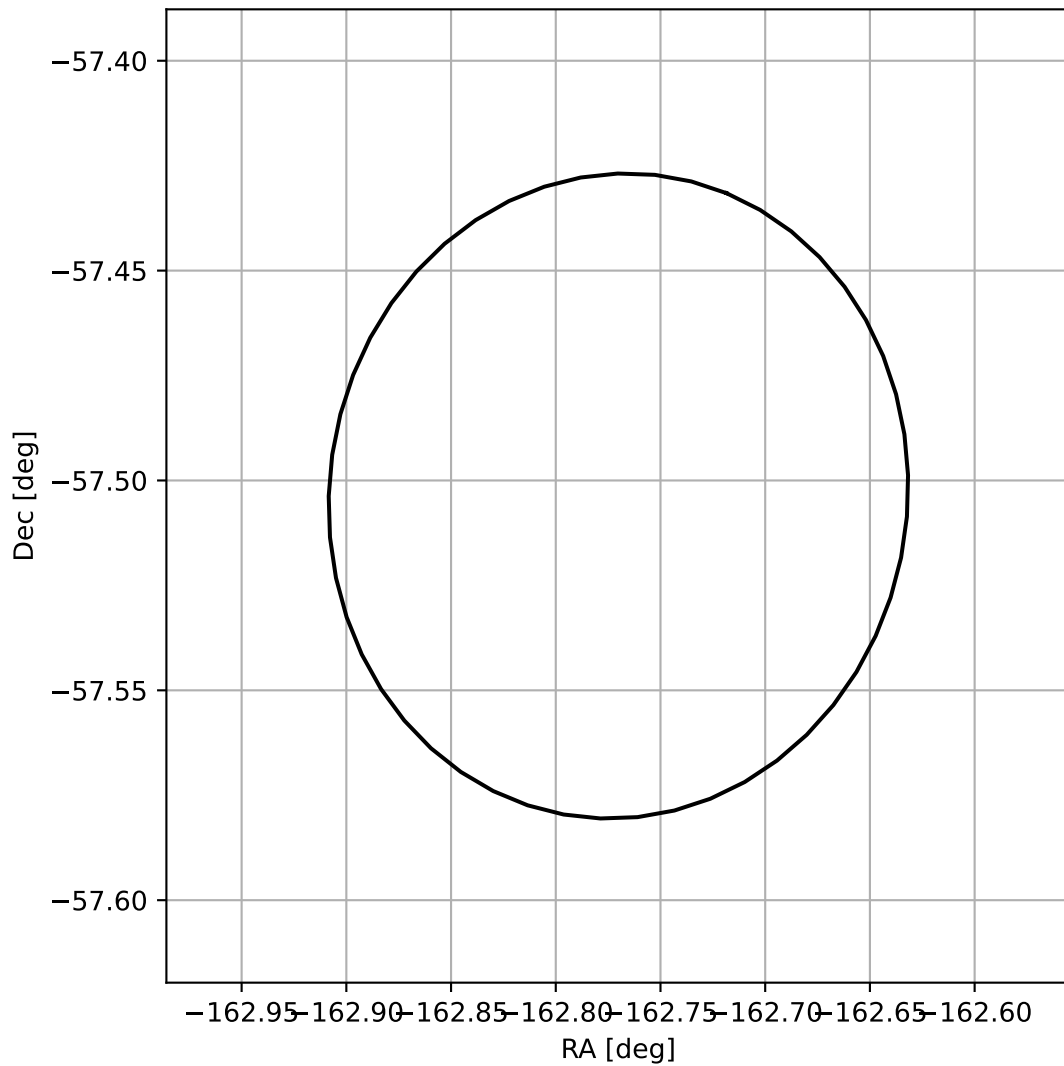
4FGL J1308.9-5730
