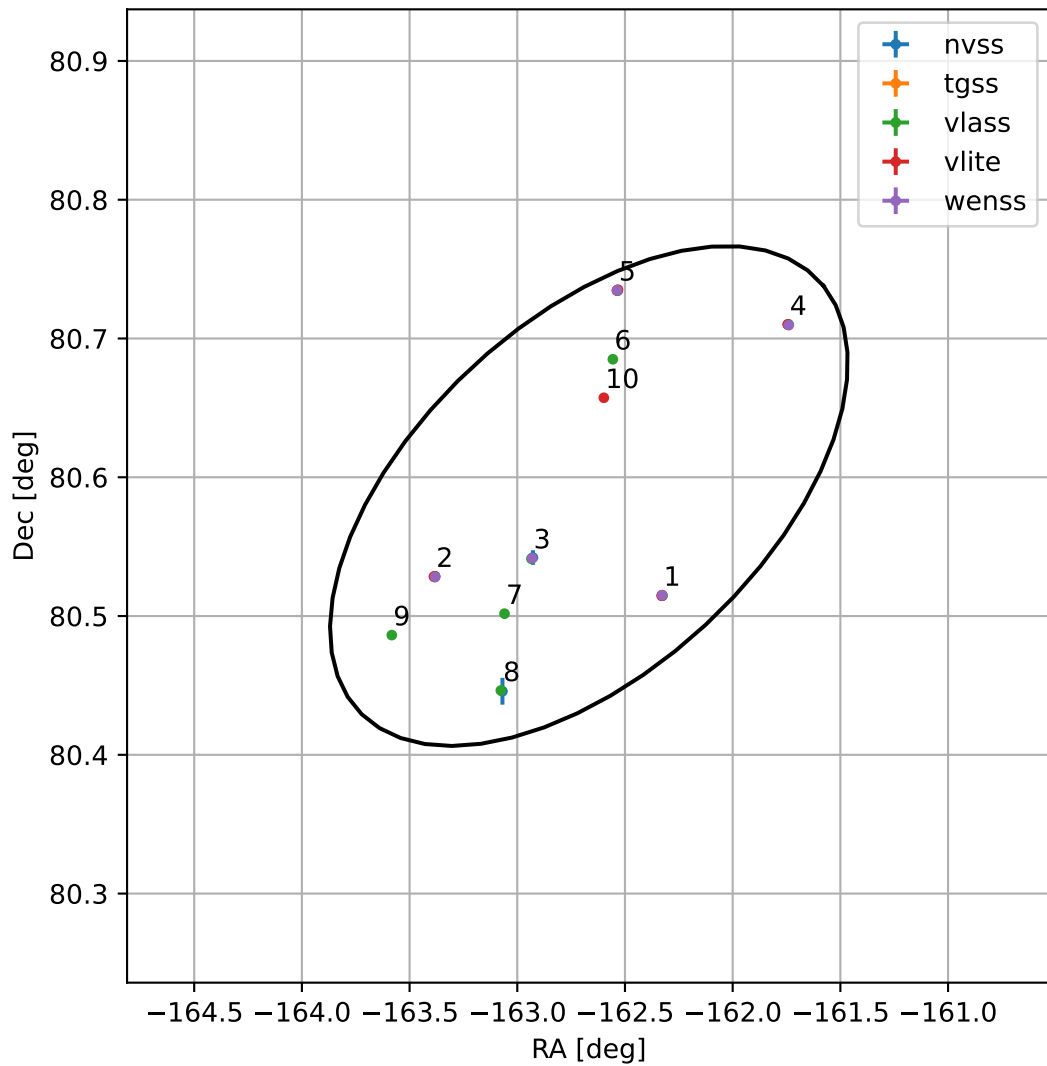
4FGL J1309.3+8035
