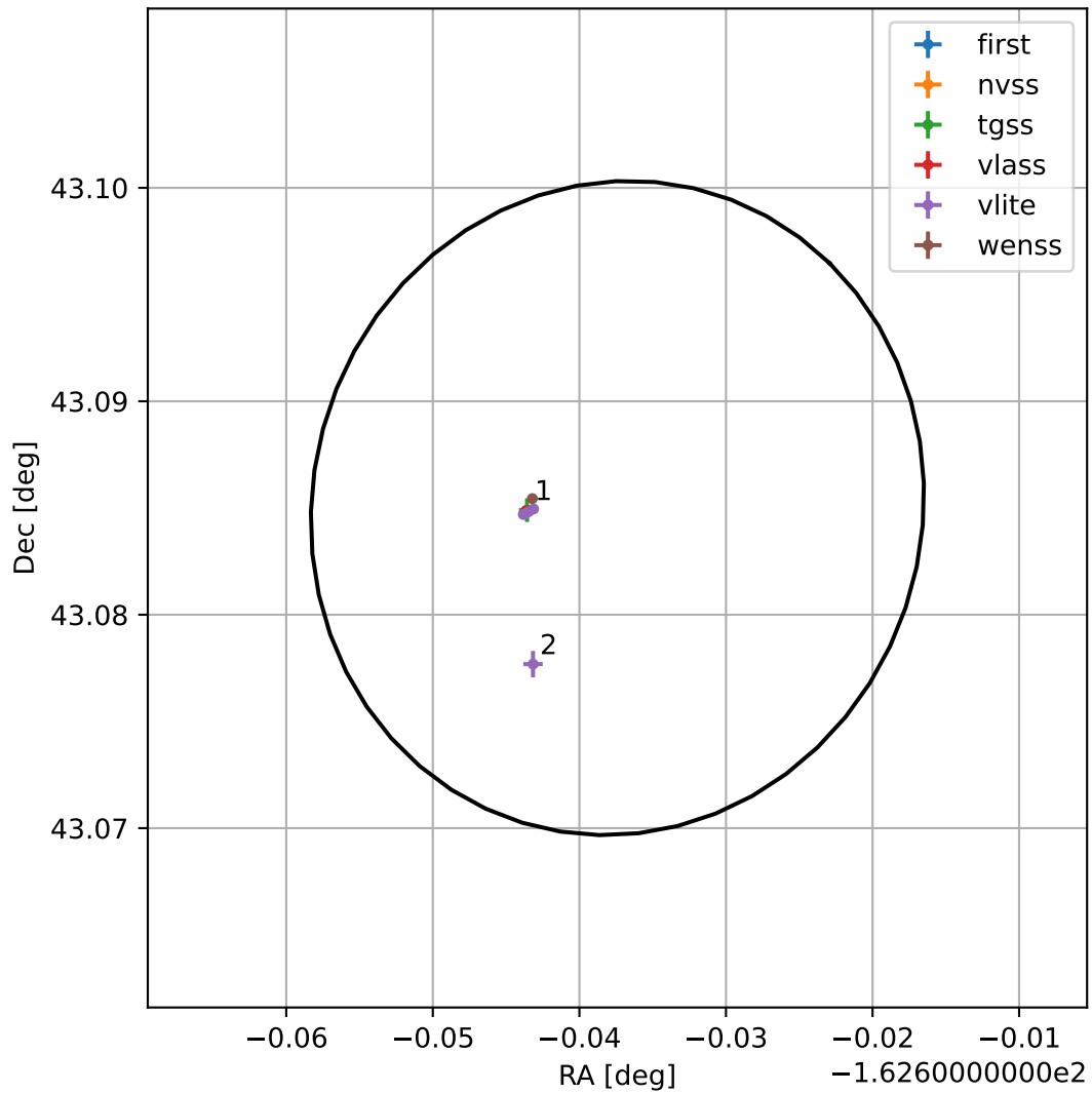
4FGL J1309.4+4305
