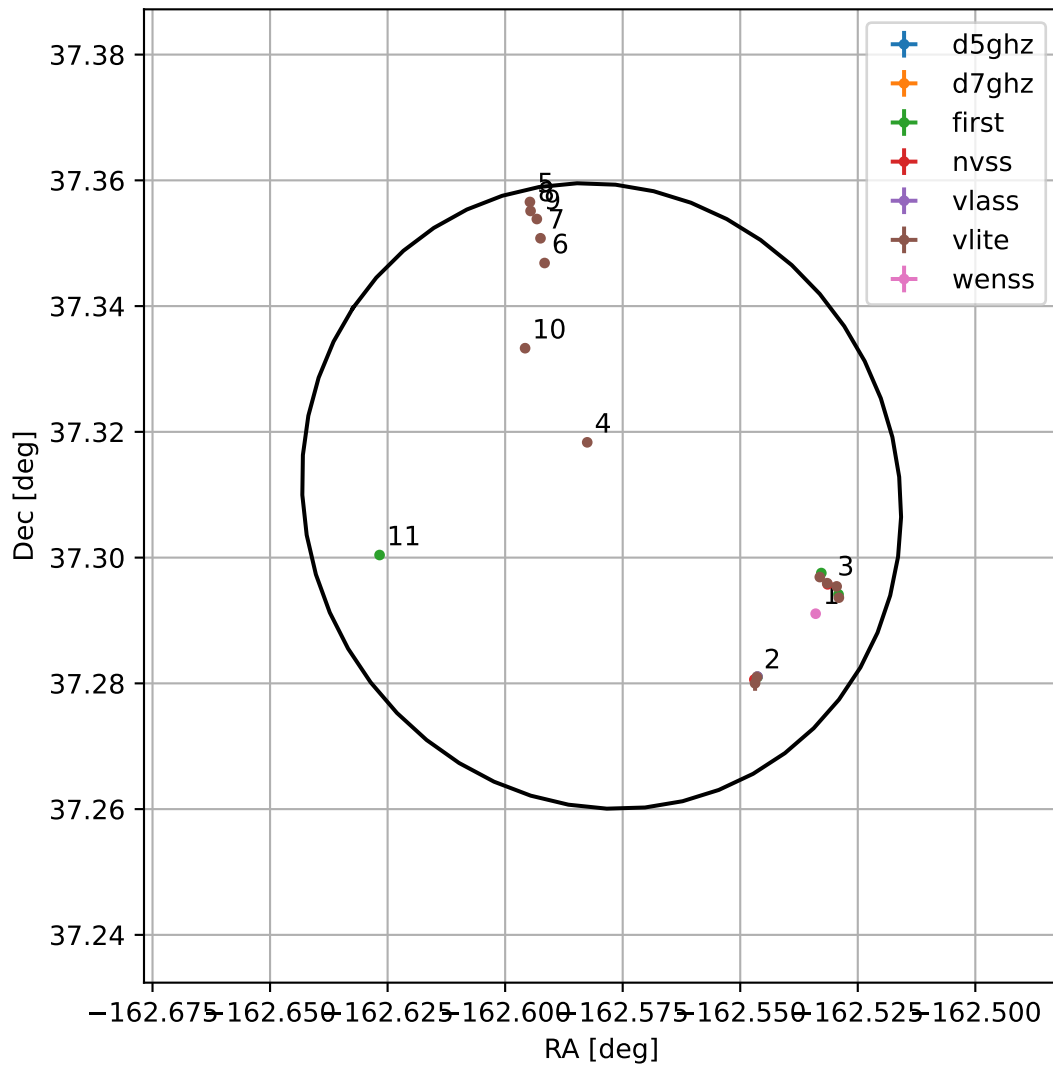
4FGL J1309.6+3718
