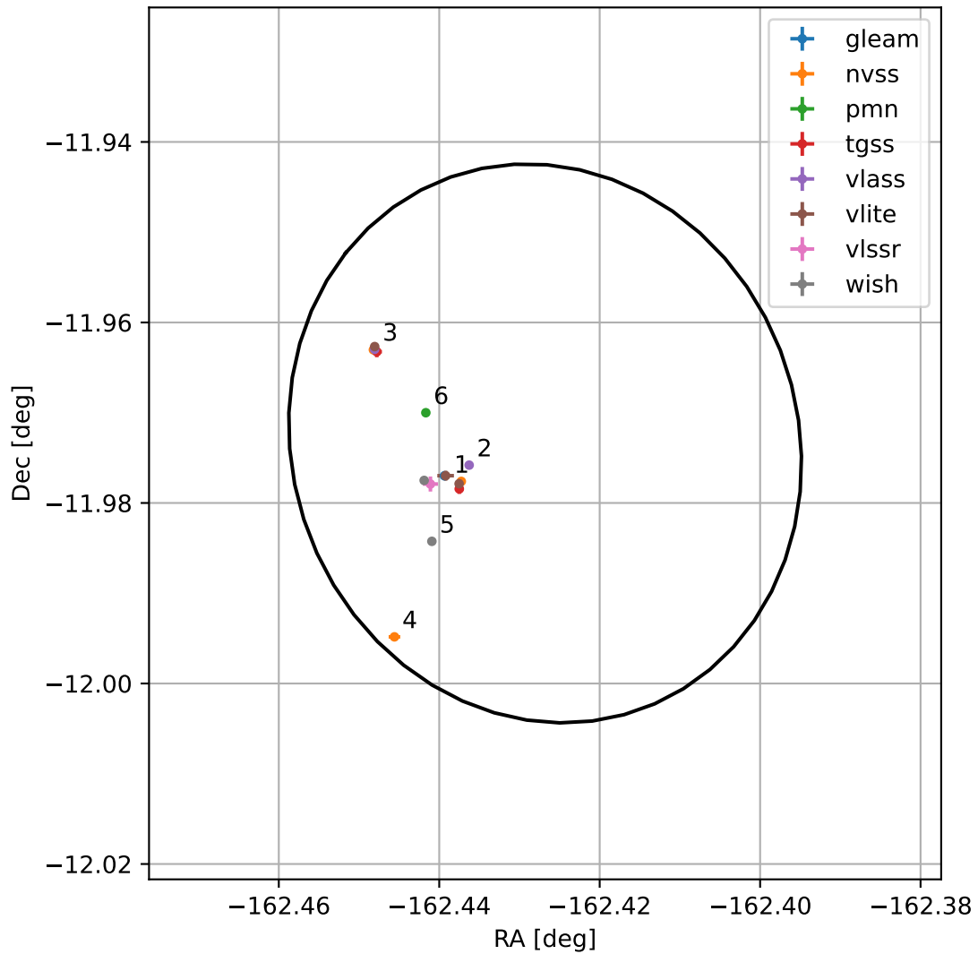
4FGL J1310.2-1158
