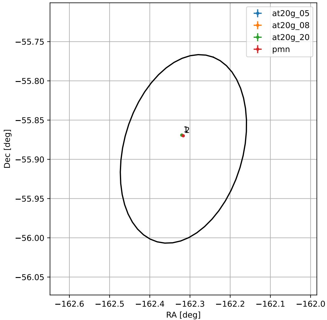
4FGL J1310.7-5553
