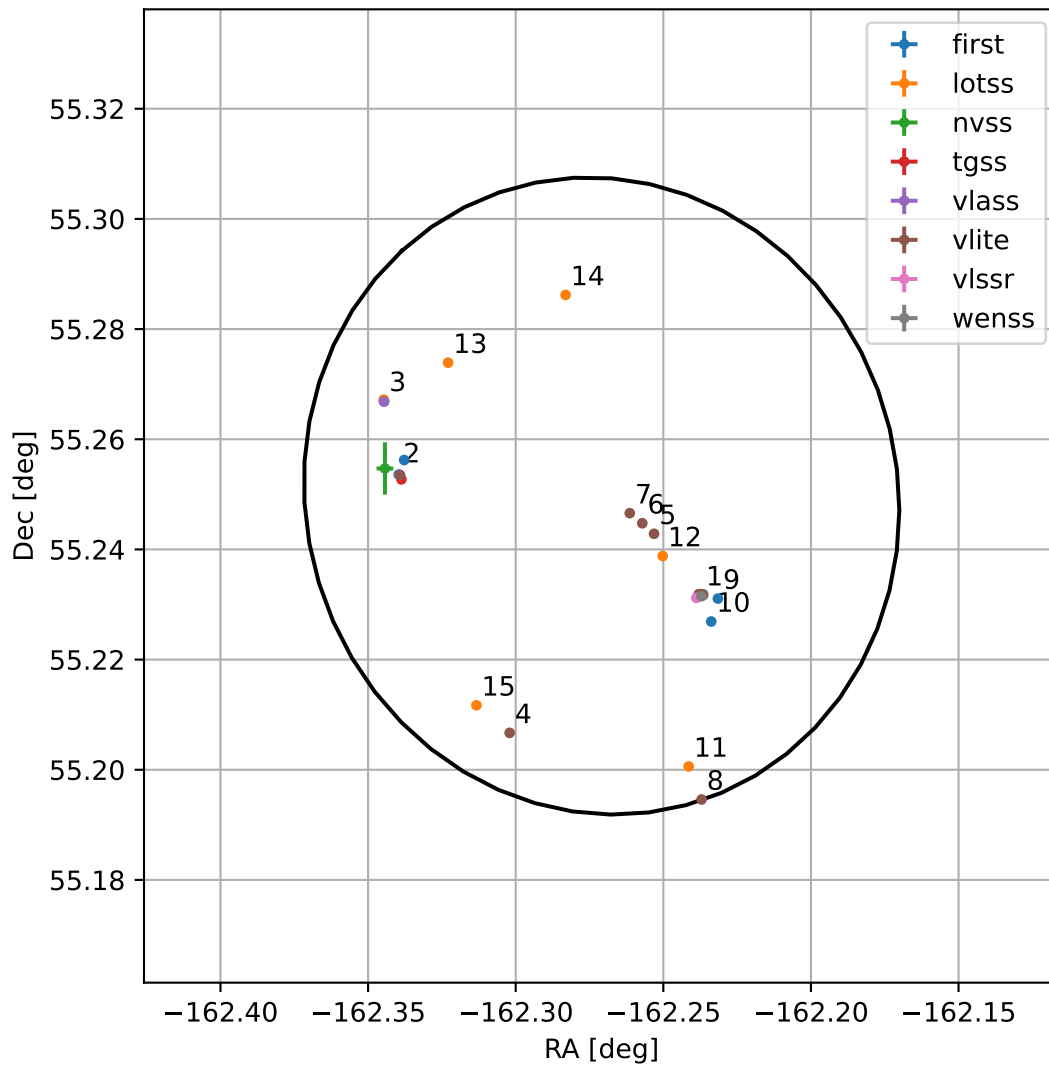
4FGL J1310.9+5514
