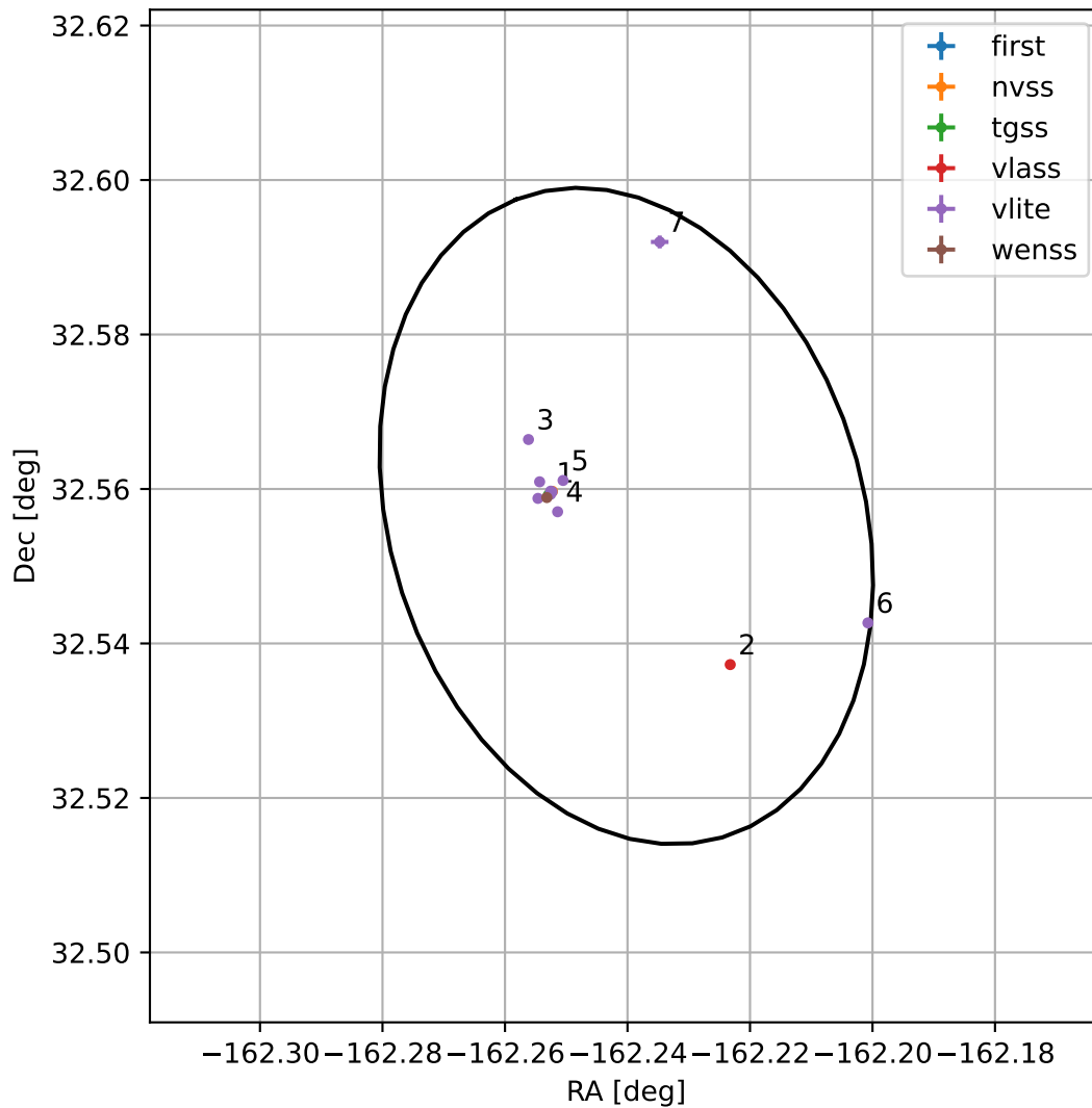
4FGL J1311.0+3233
