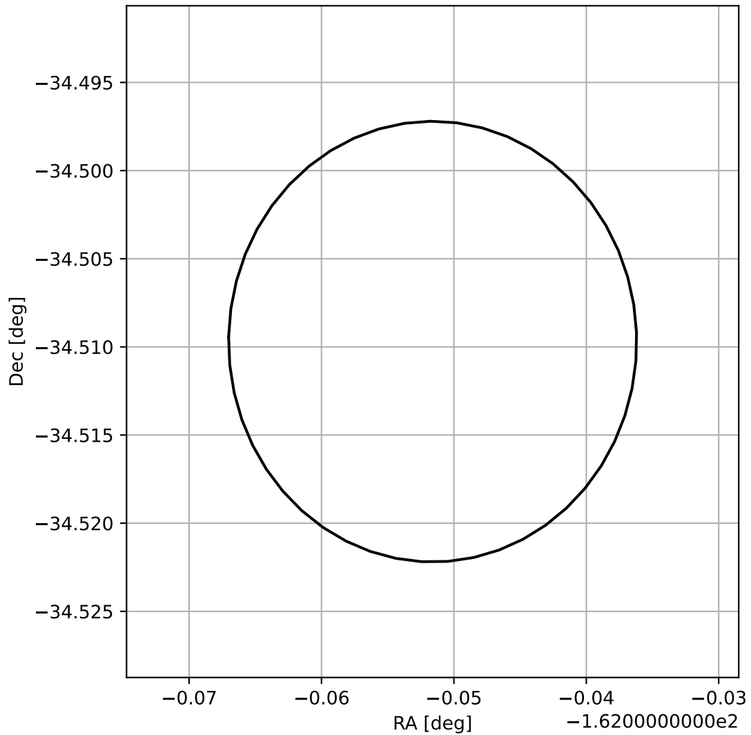
4FGL J1311.7-3430
