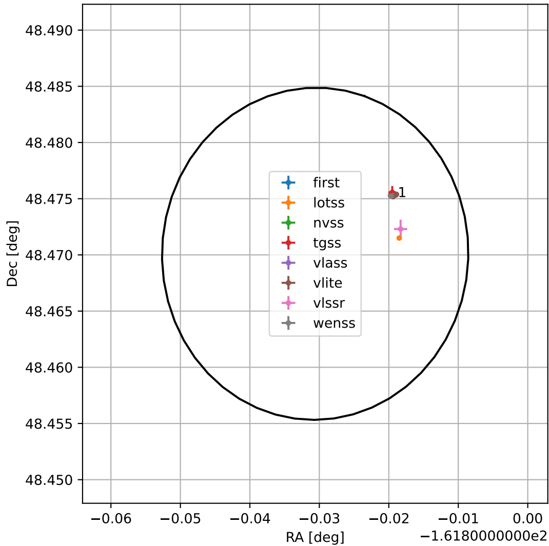
4FGL J1312.6+4828
