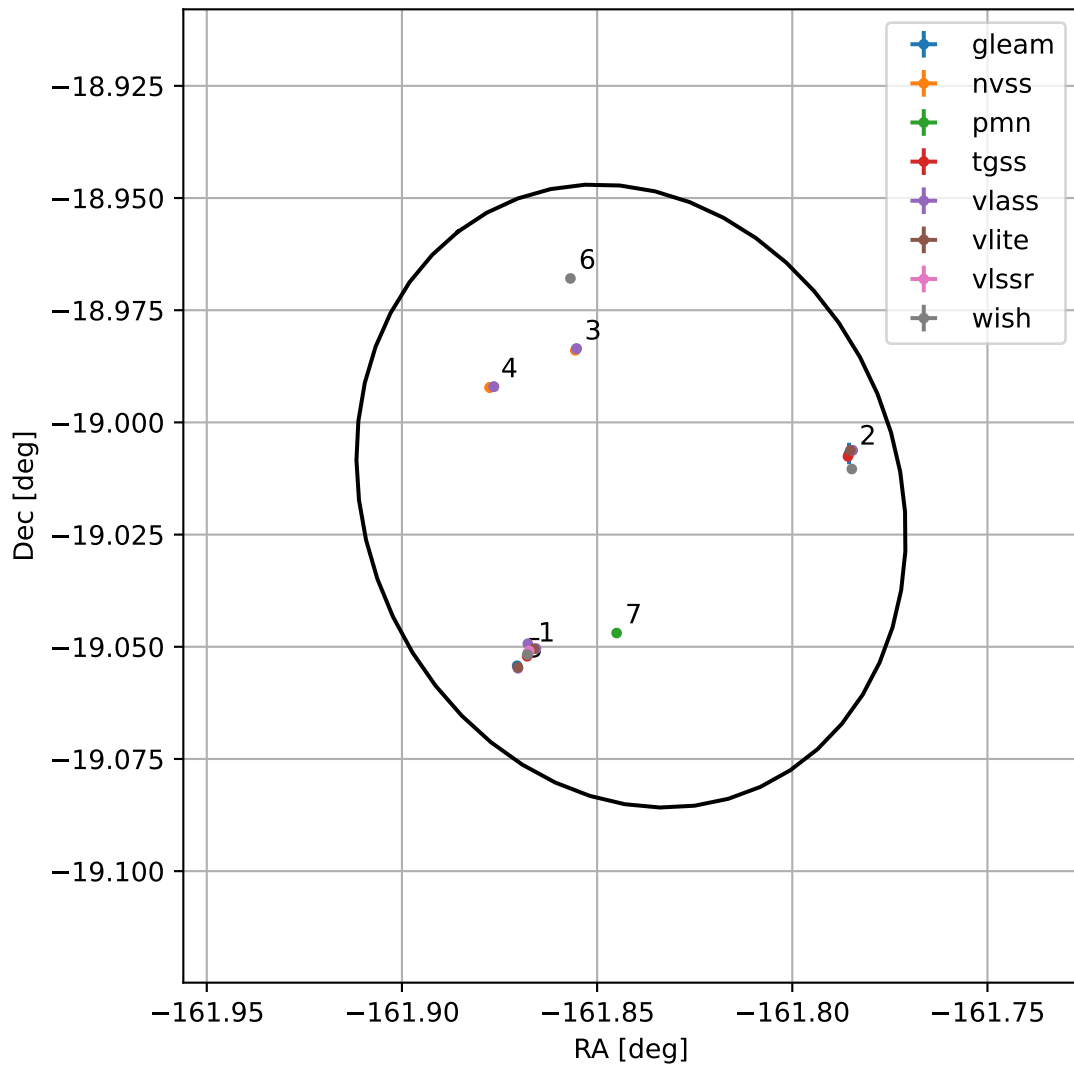
4FGL J1312.6-1900
