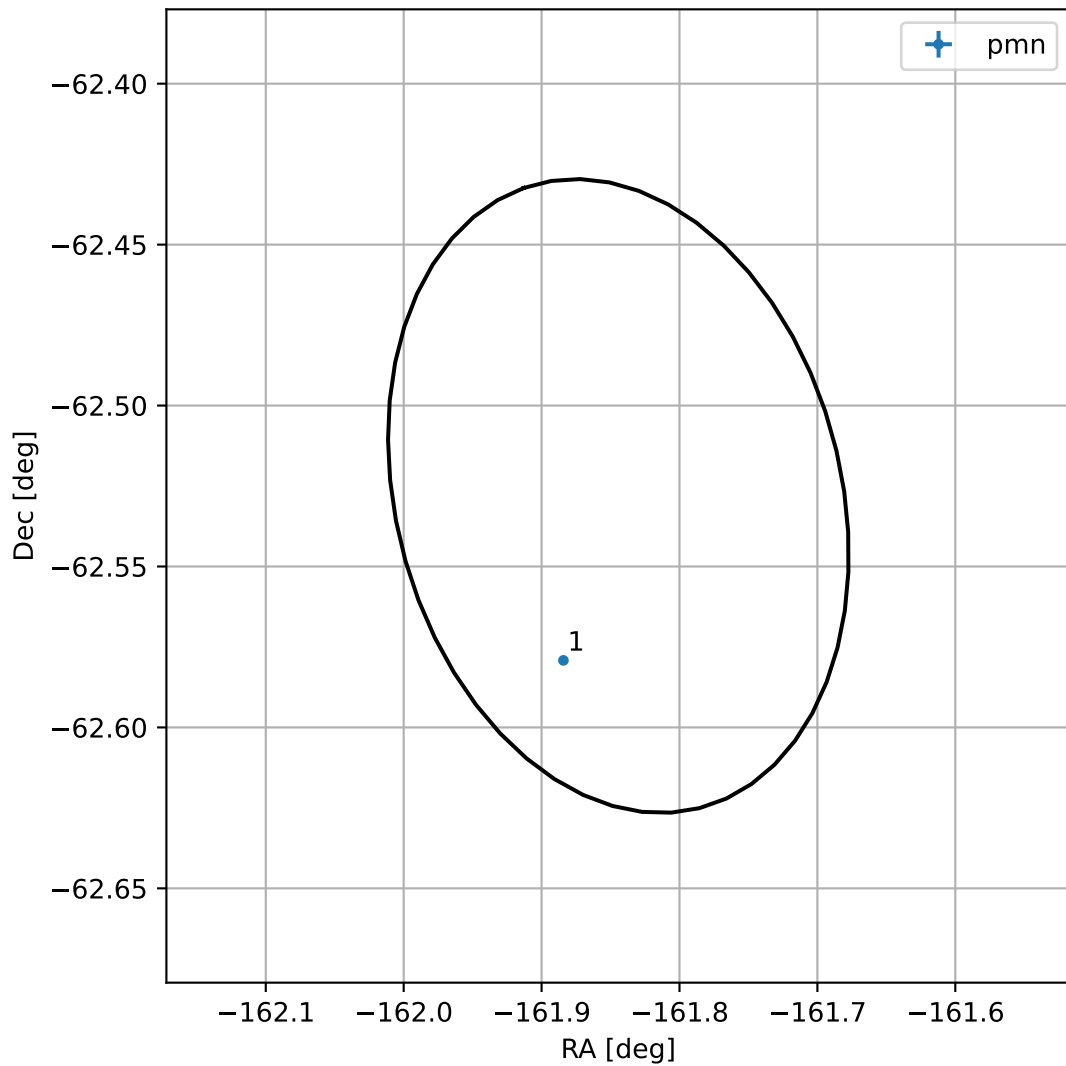
4FGL J1312.6-6231
