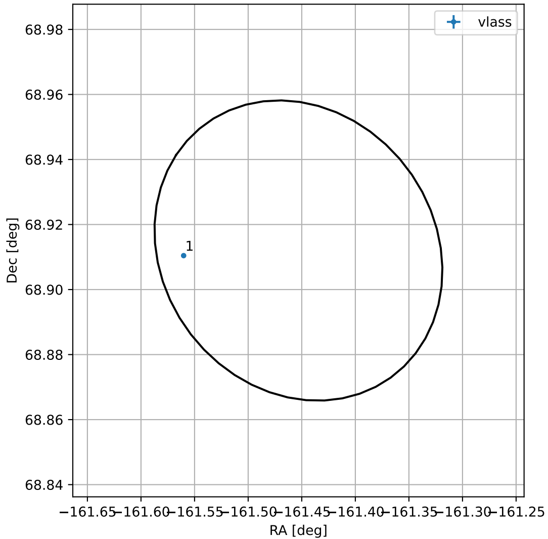
4FGL J1314.1+6854
