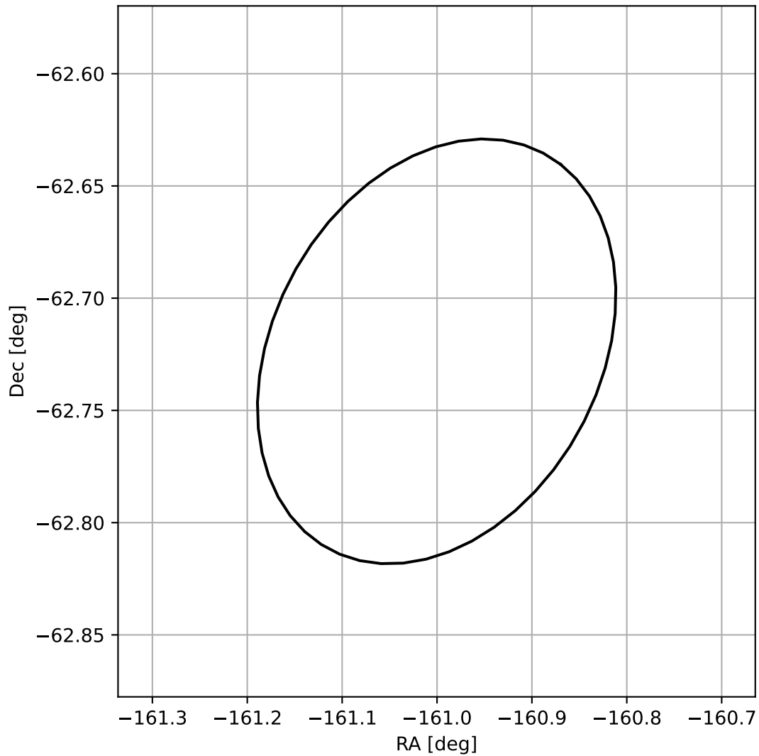
4FGL J1315.9-6243
