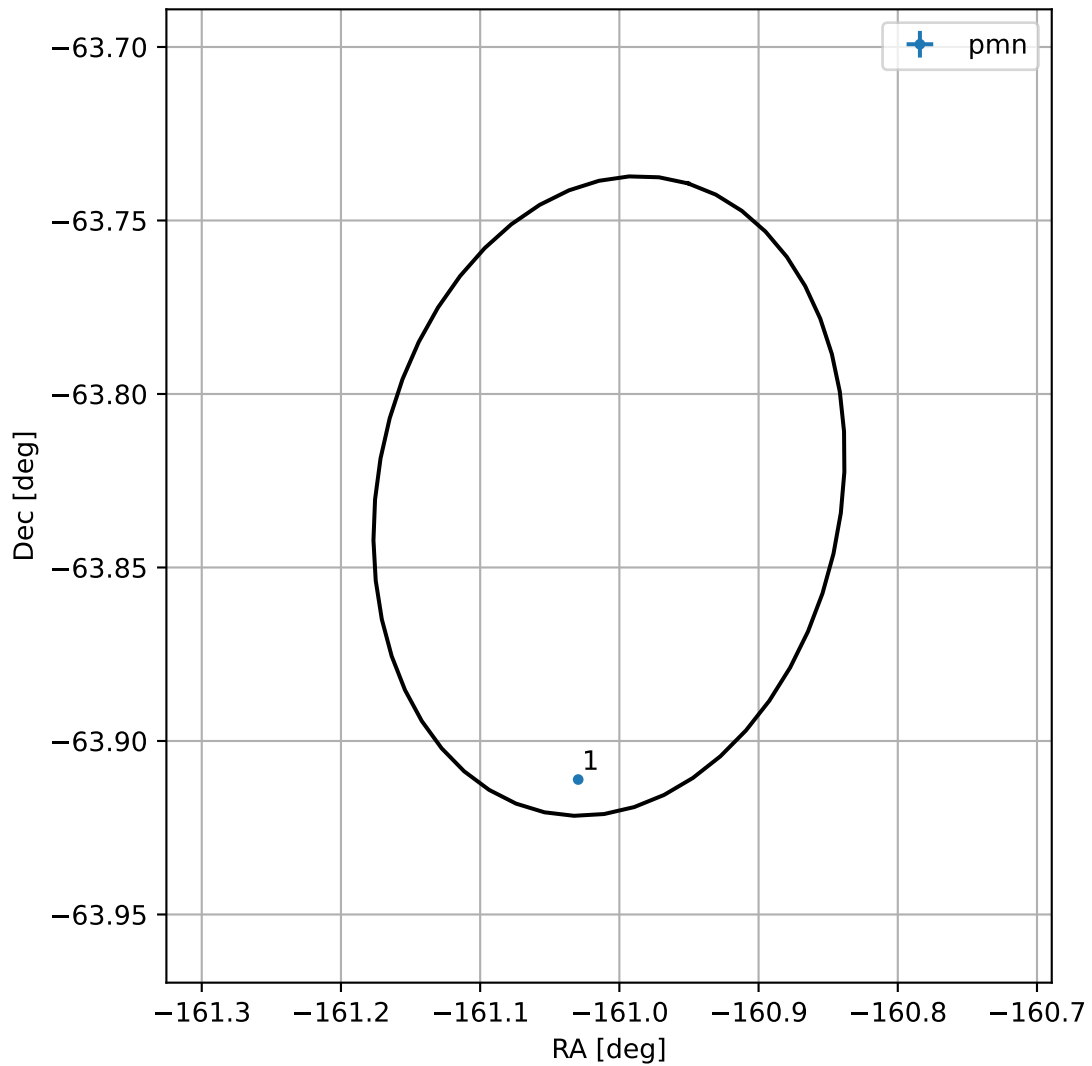
4FGL J1315.9-6349
