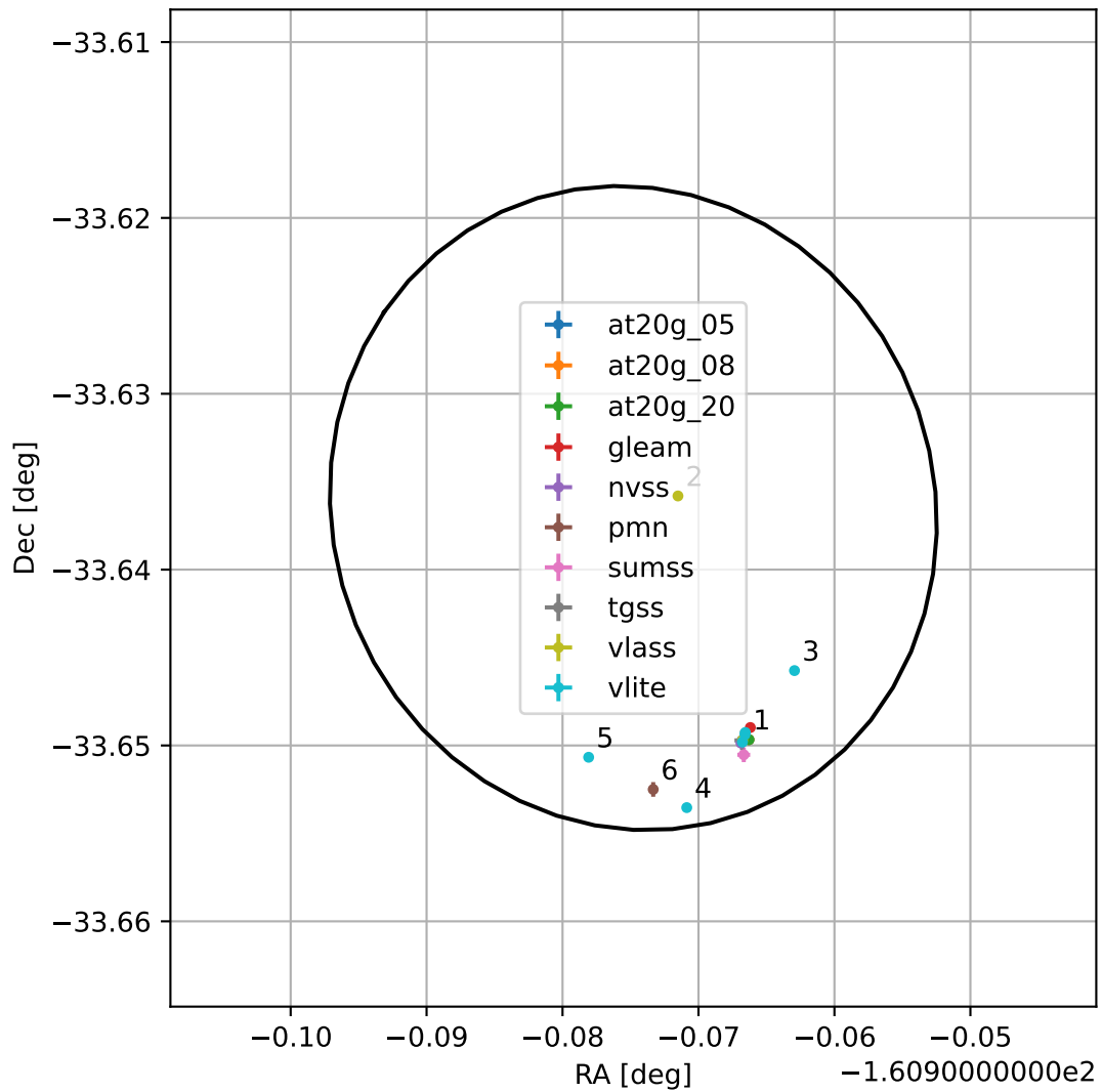
4FGL J1316.1-3338
