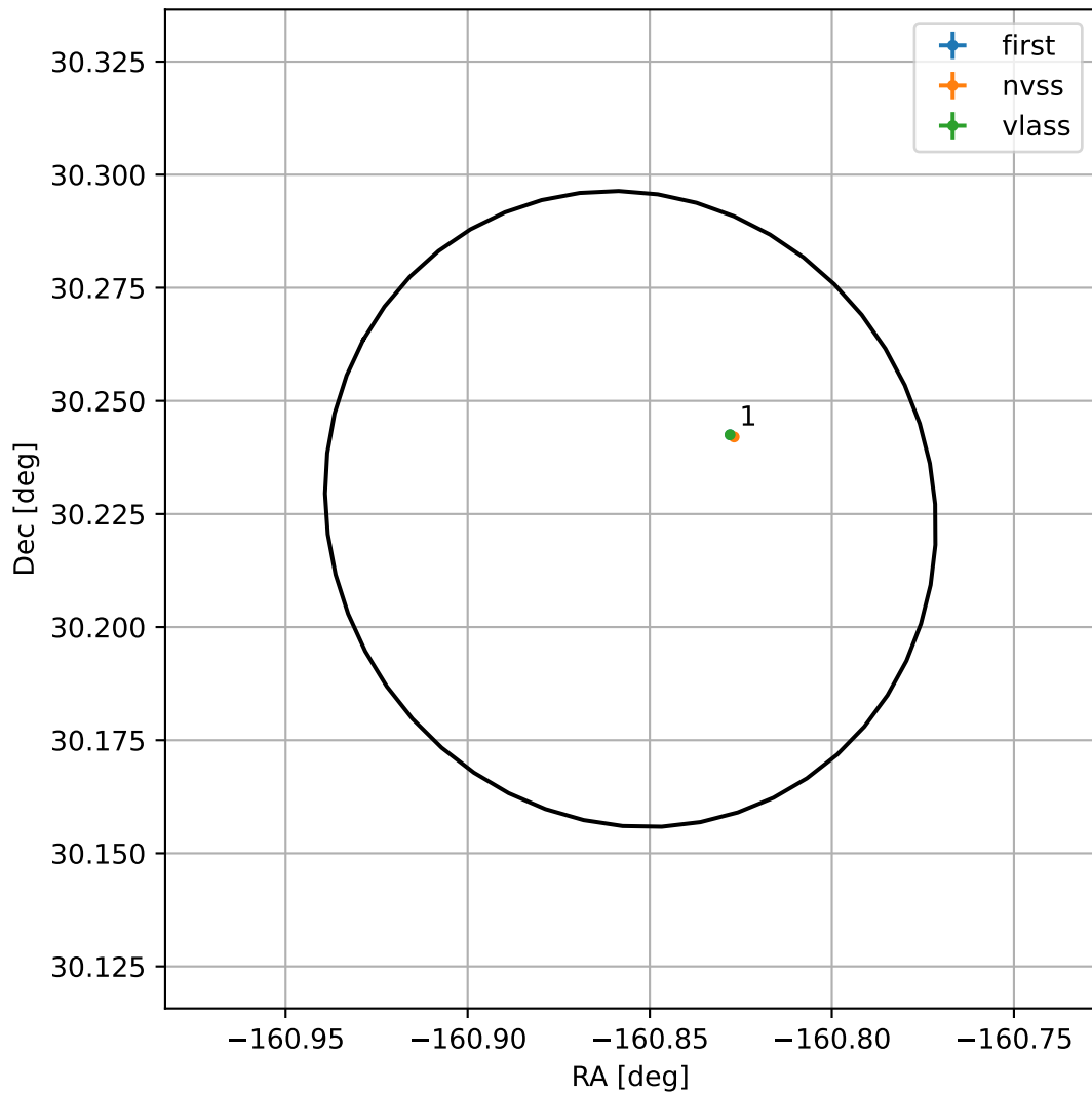
4FGL J1316.5+3013
