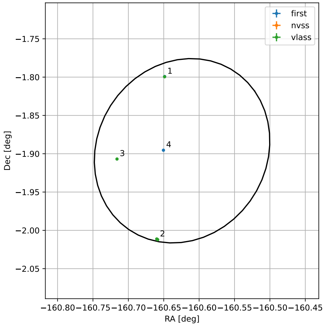
4FGL J1317.5-0153
