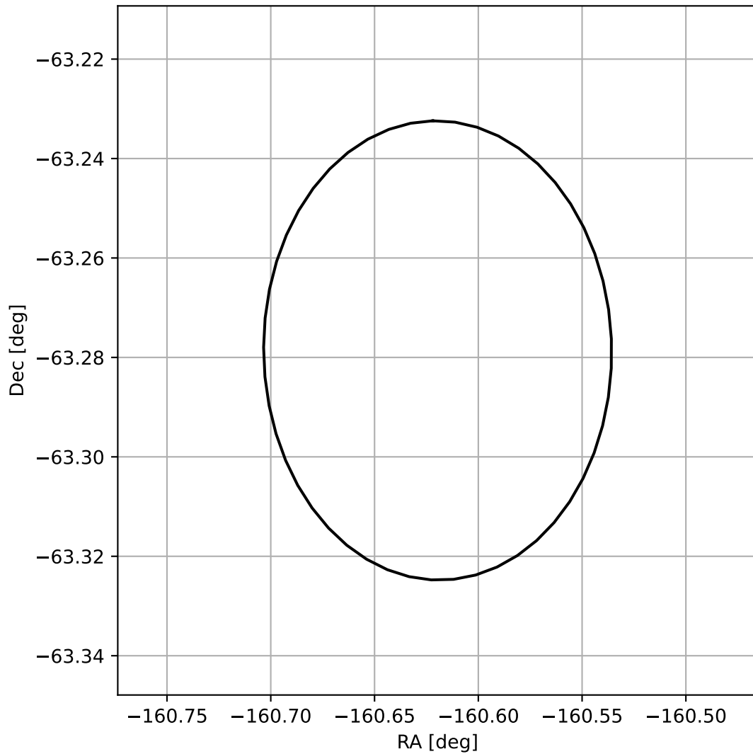
4FGL J1317.5-6316
