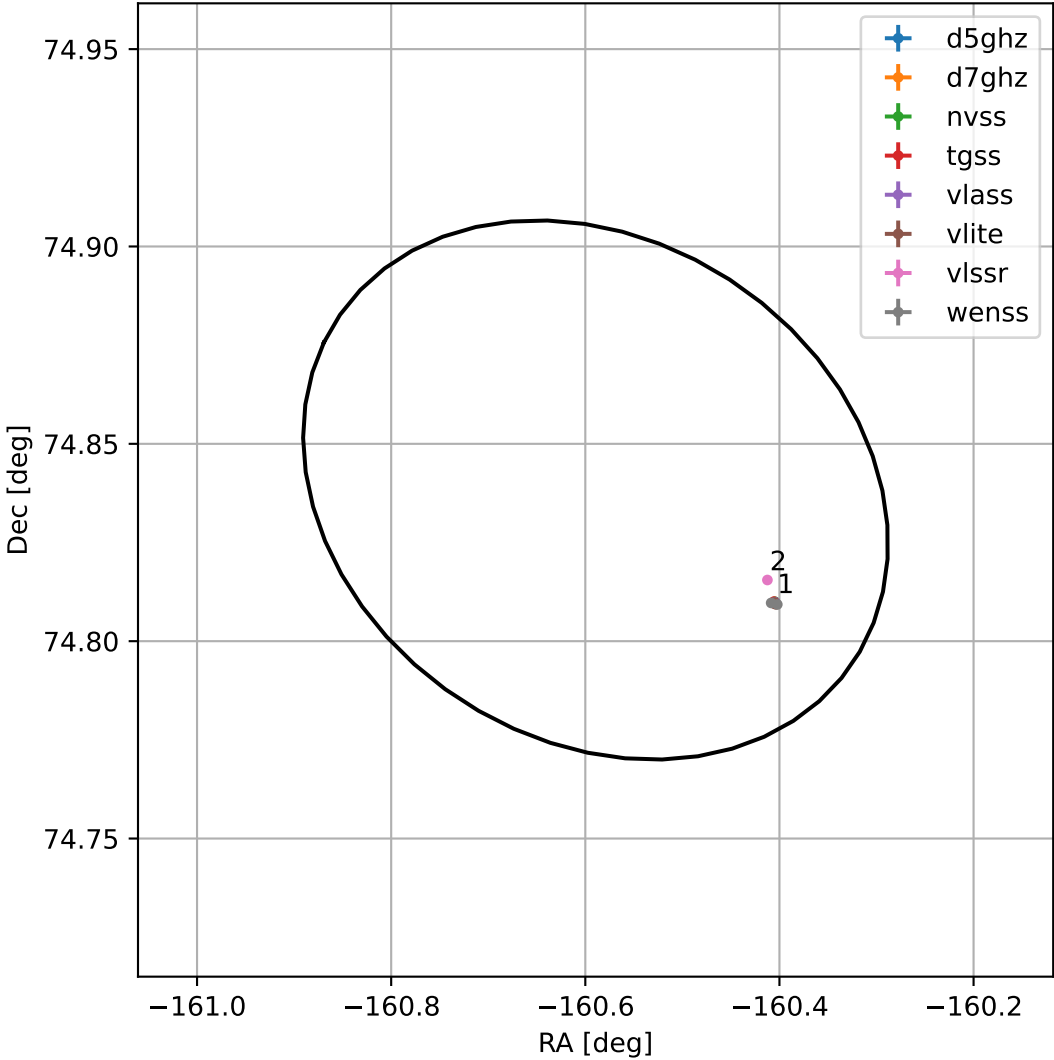
4FGL J1317.6+7450
