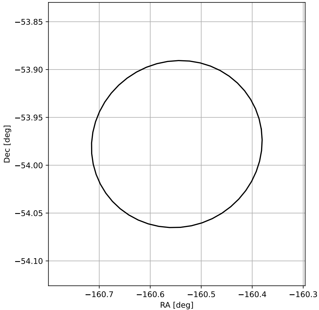
4FGL J1317.8-5358
