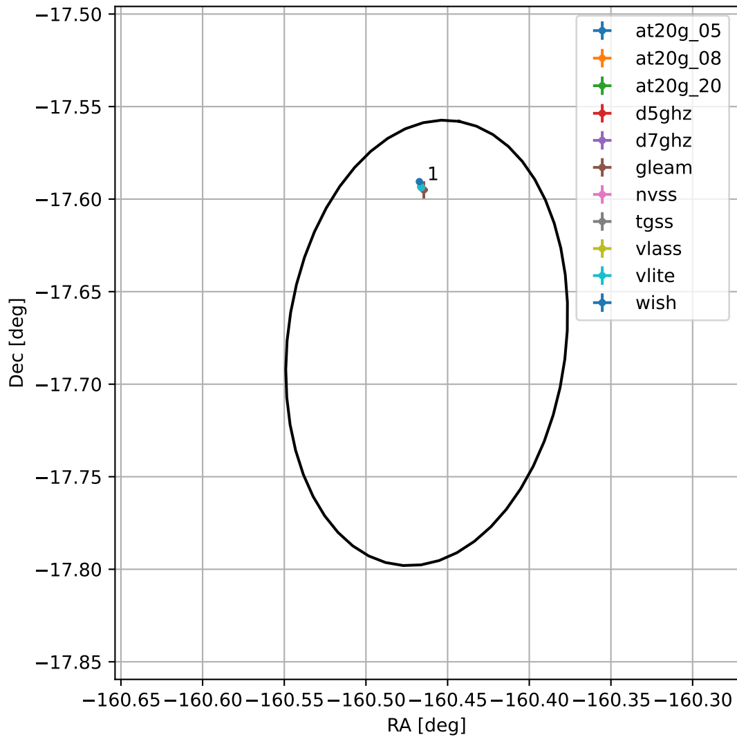
4FGL J1318.1-1740
