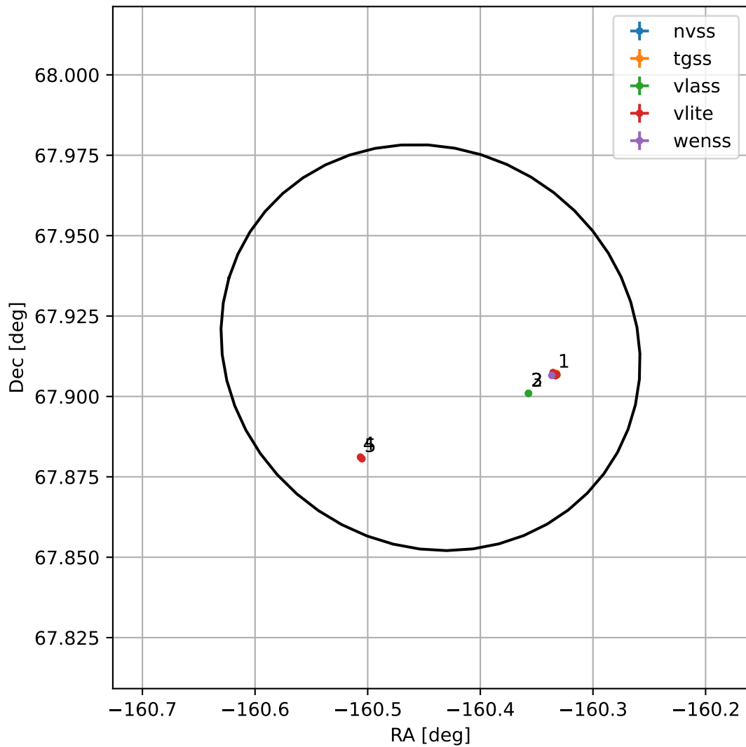
4FGL J1318.2+6754
