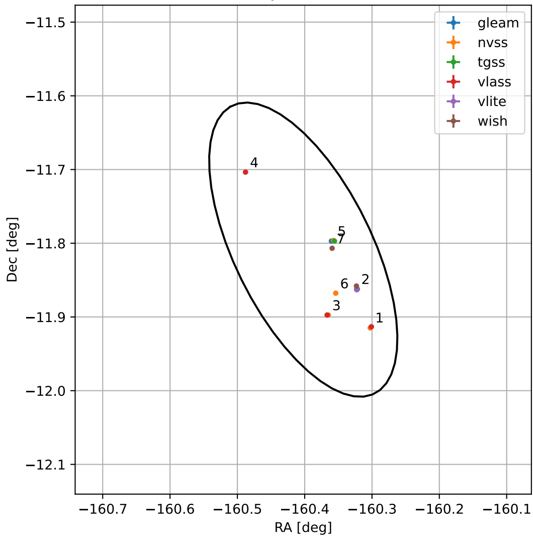
4FGL J1318.3-1148
