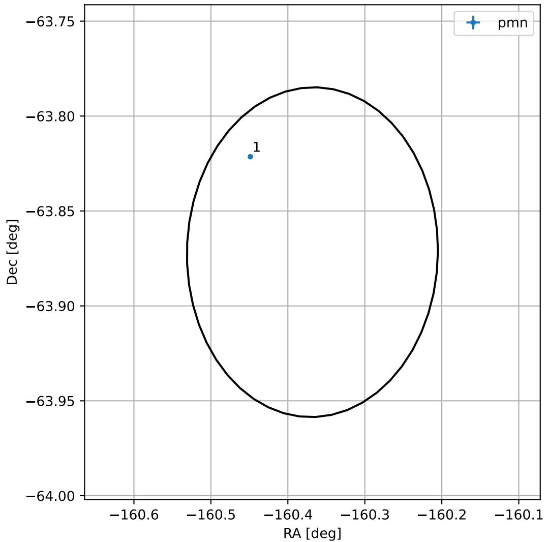
4FGL J1318.5-6352
