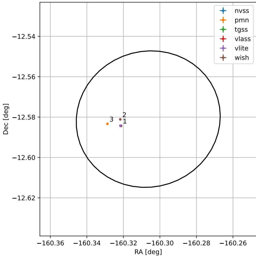
4FGL J1318.7-1234
