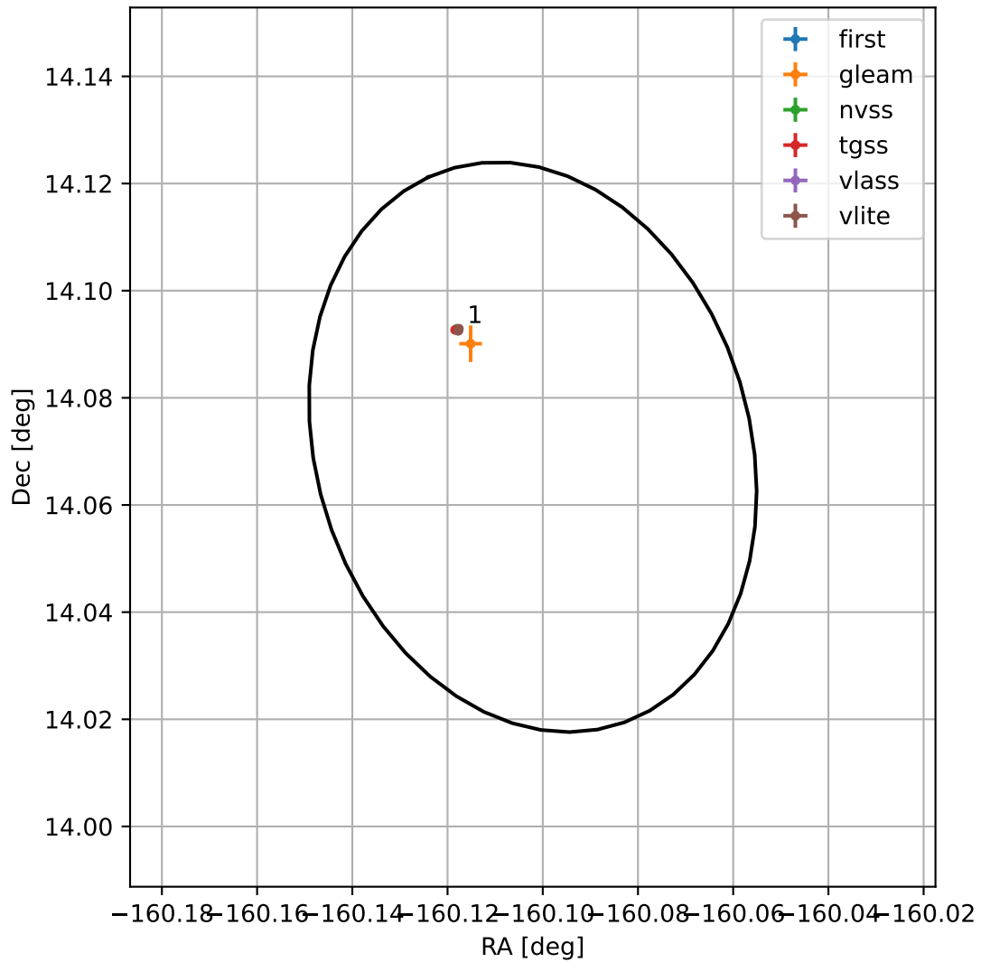
4FGL J1319.5+1404
