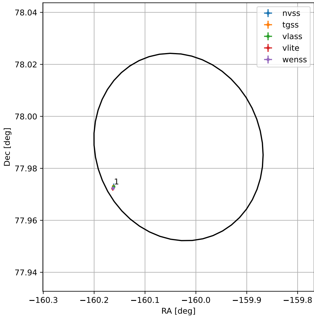
4FGL J1319.8+7759
