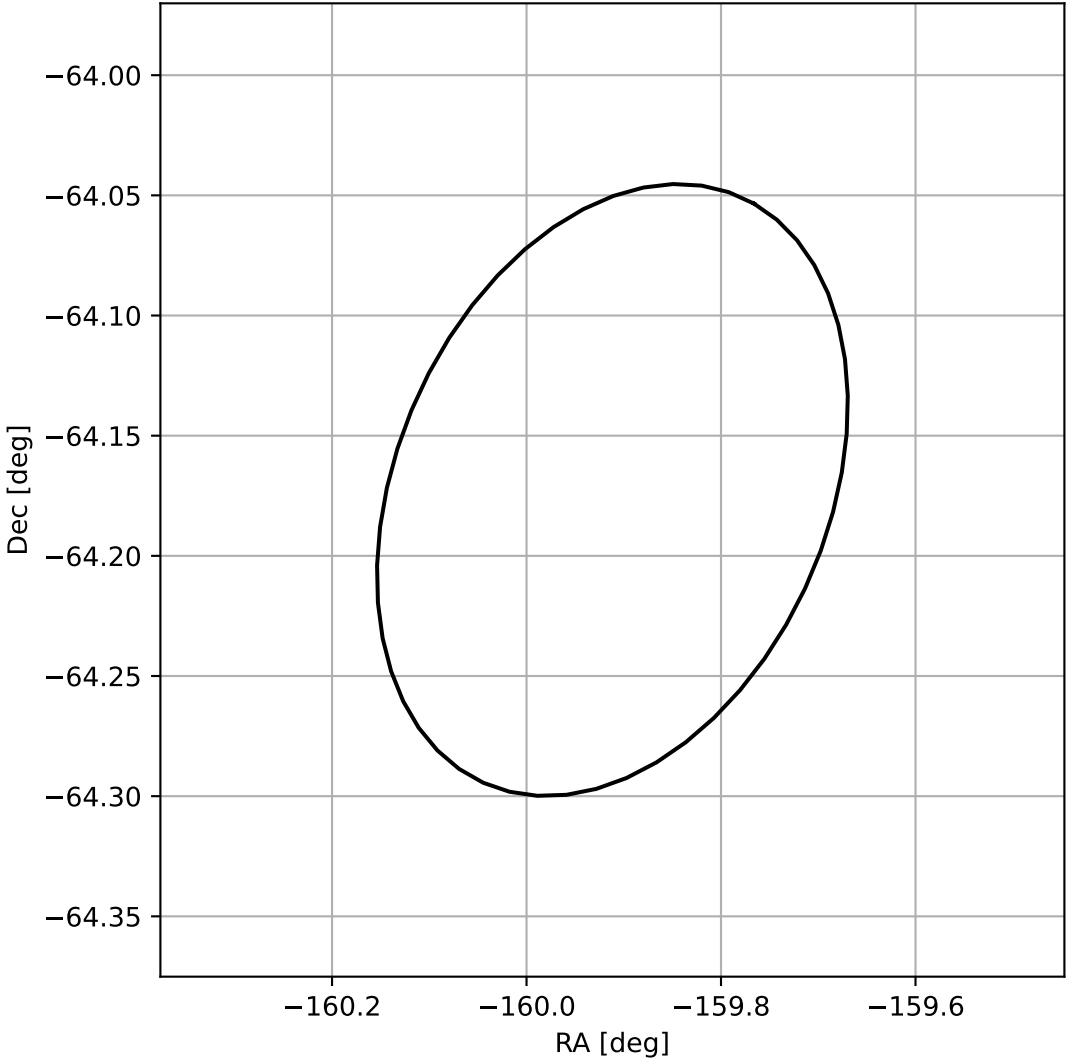
4FGL J1320.3-6410
