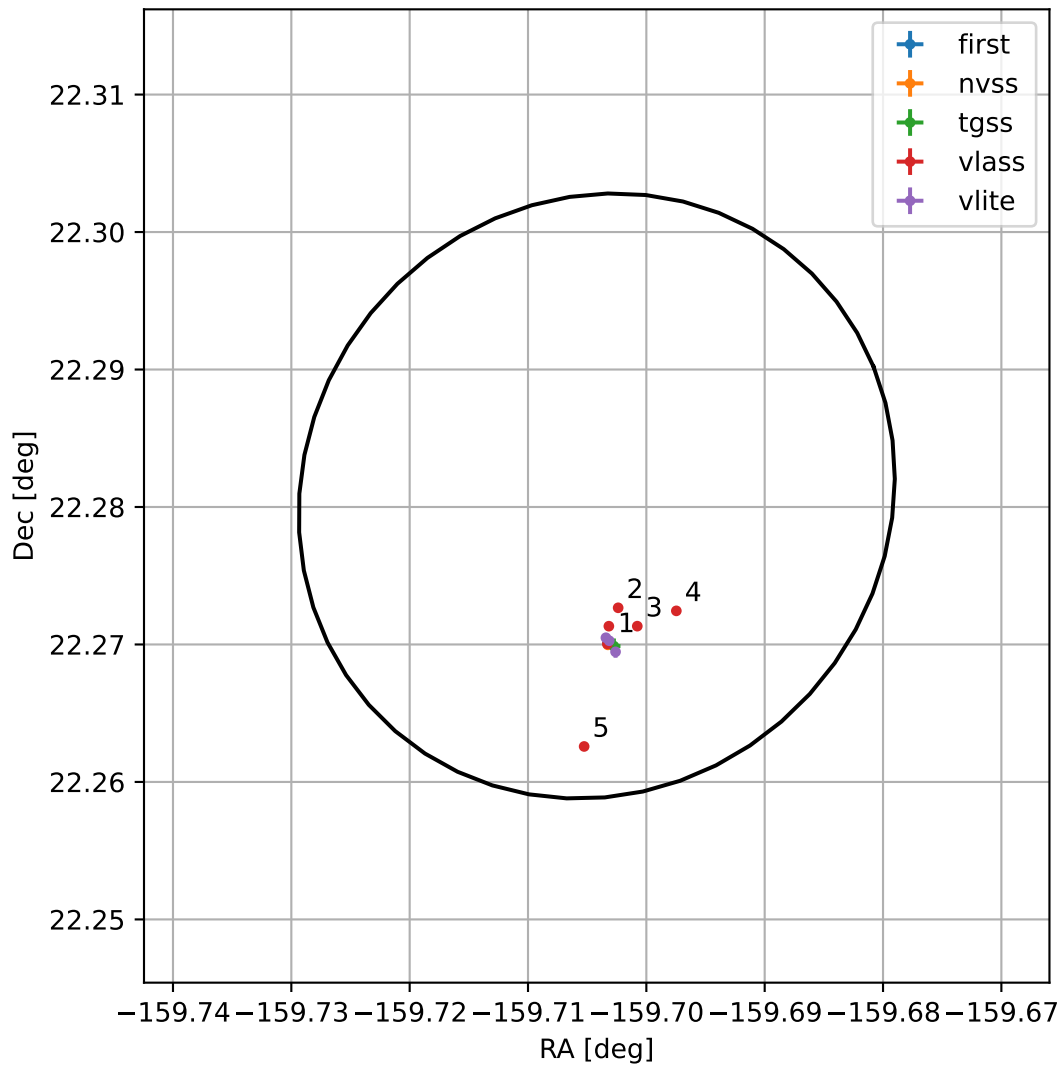
4FGL J1321.1+2216
