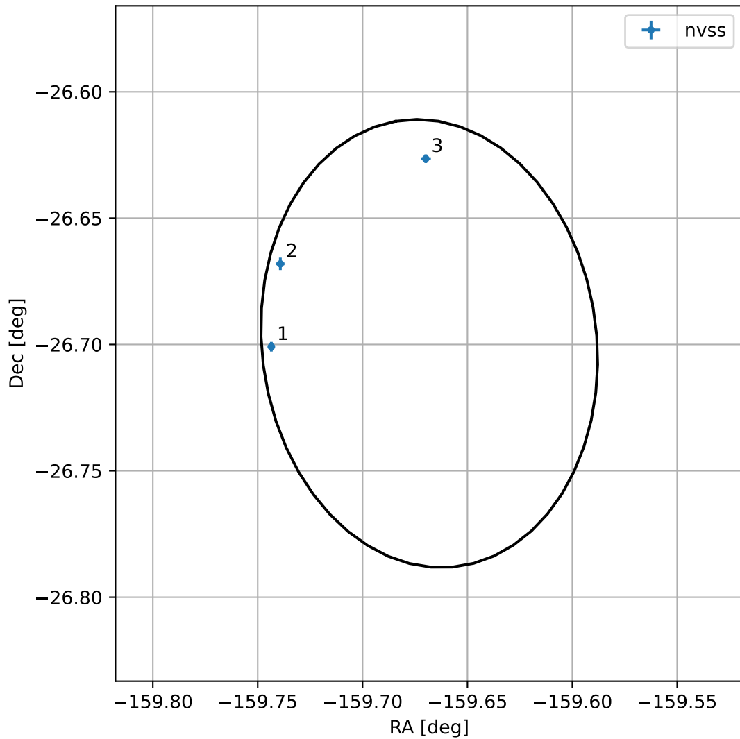
4FGL J1321.3-2641
