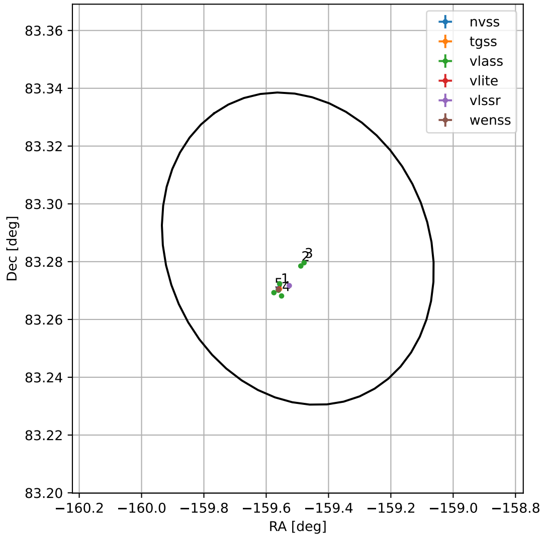
4FGL J1322.0+8317
