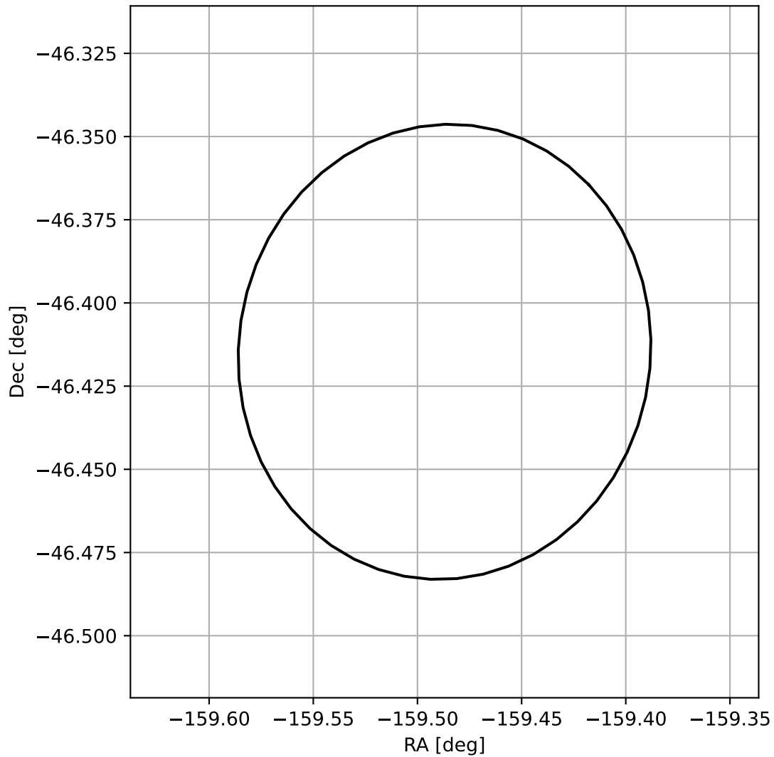
4FGL J1322.0-4624
