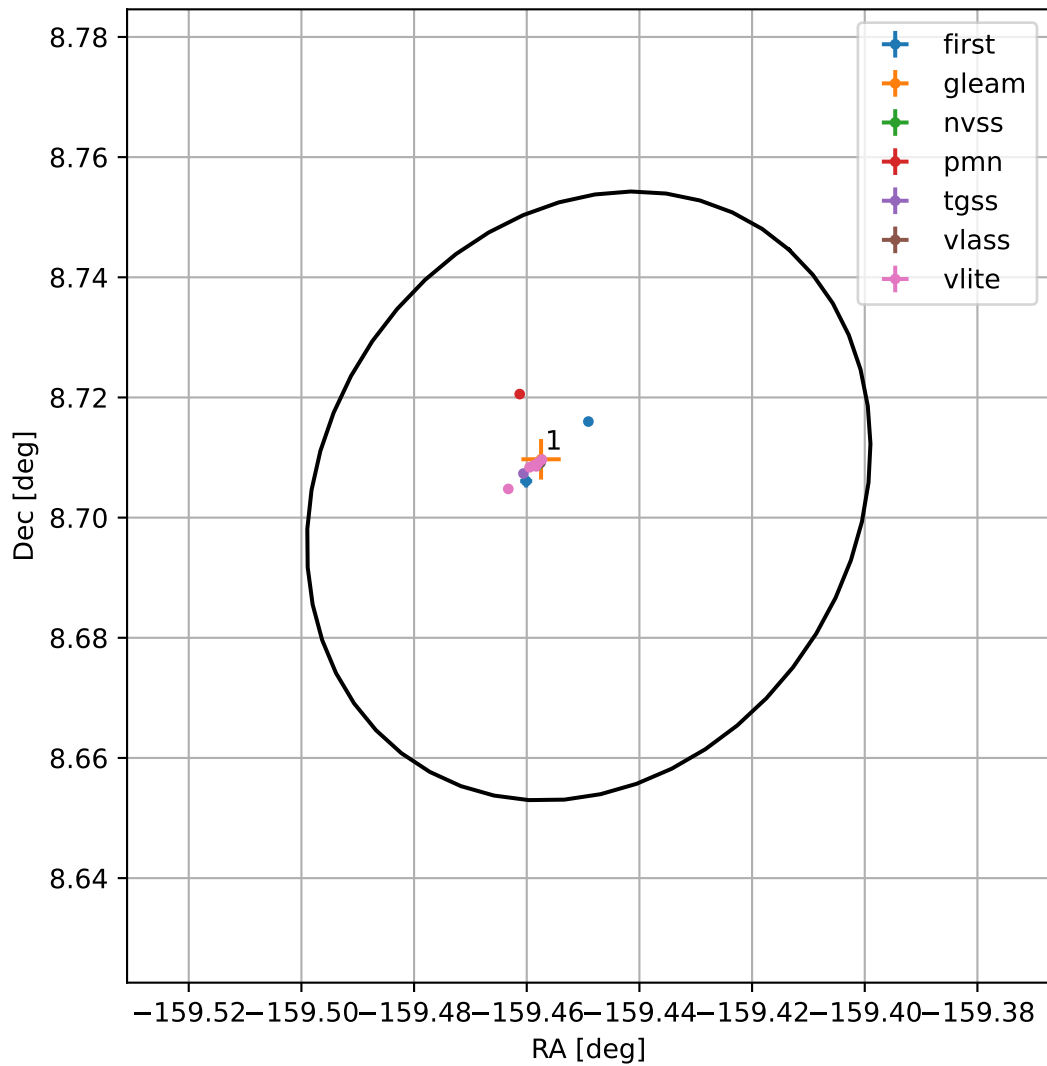
4FGL J1322.2+0842
