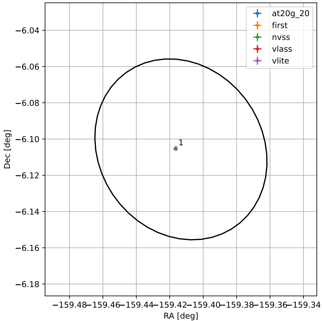
4FGL J1322.3-0606
