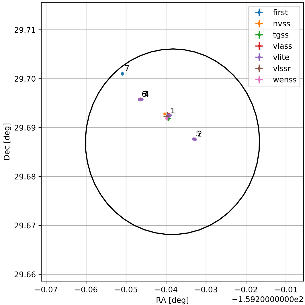
4FGL J1323.0+2941
