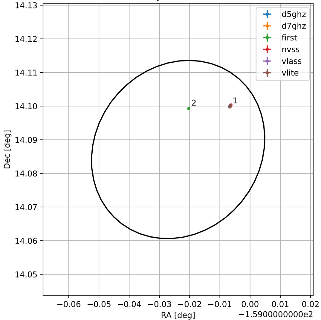
4FGL J1323.9+1405
