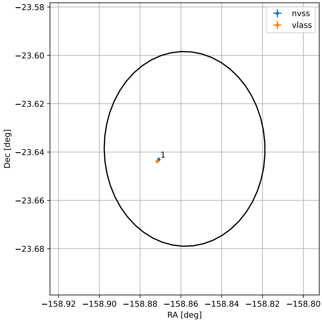
4FGL J1324.5-2338
