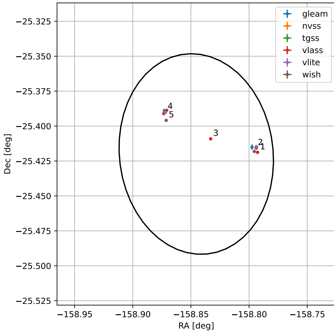
4FGL J1324.6-2525
