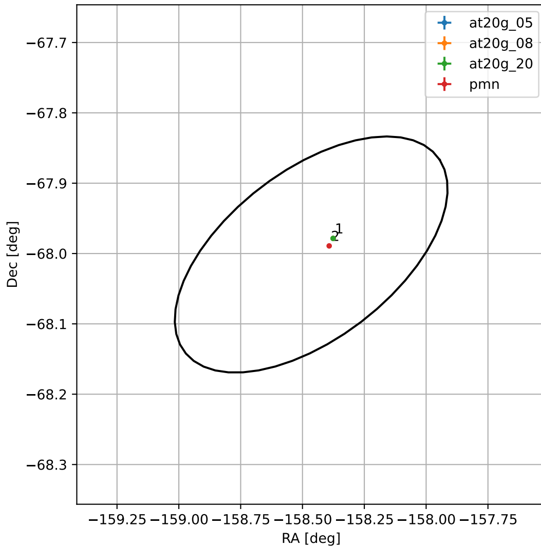
4FGL J1326.1-6800
