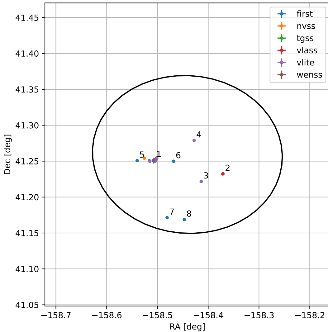
4FGL J1326.2+4115
