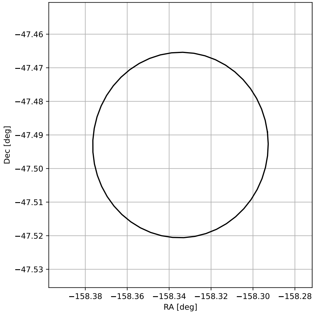
4FGL J1326.6-4729
