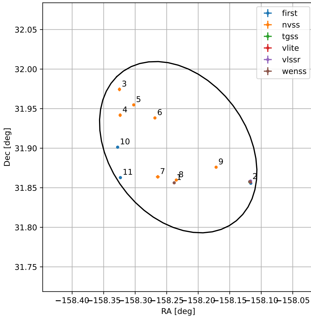
4FGL J1327.0+3154
