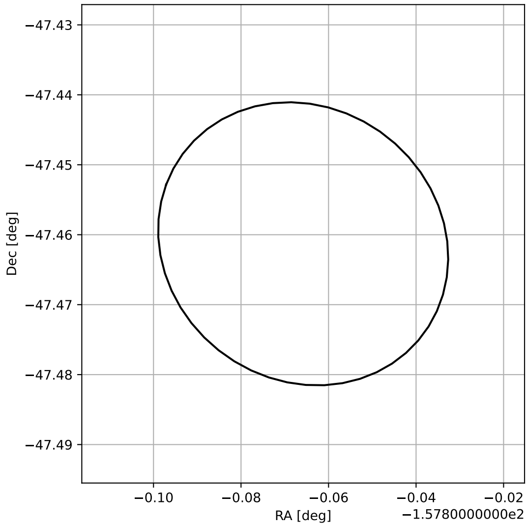
4FGL J1328.5-4727
