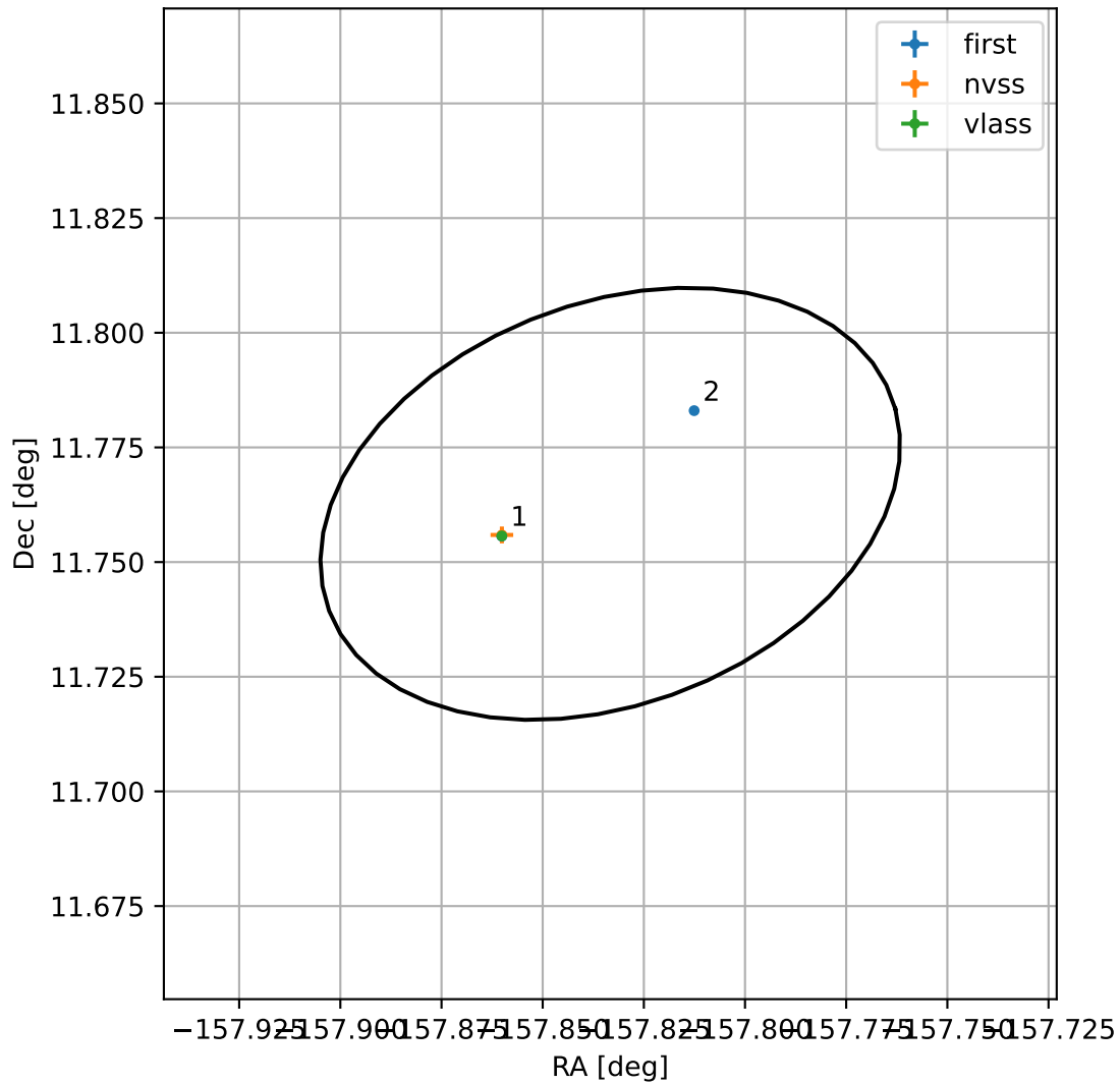
4FGL J1328.6+1145
