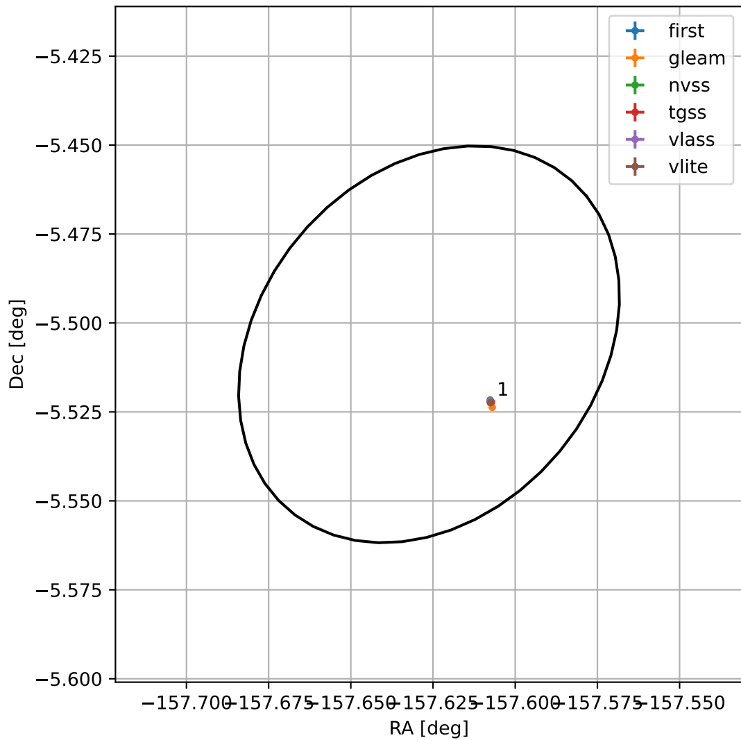
4FGL J1329.4-0530
