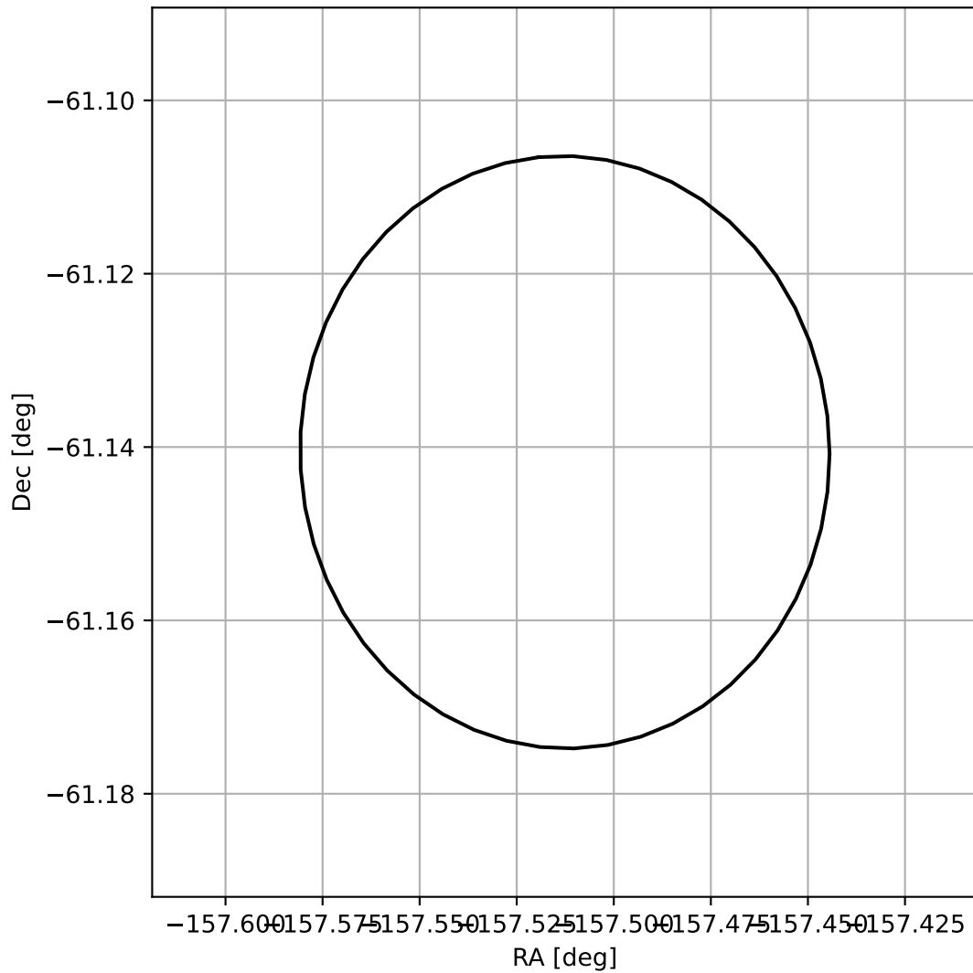
4FGL J1329.9-6108
