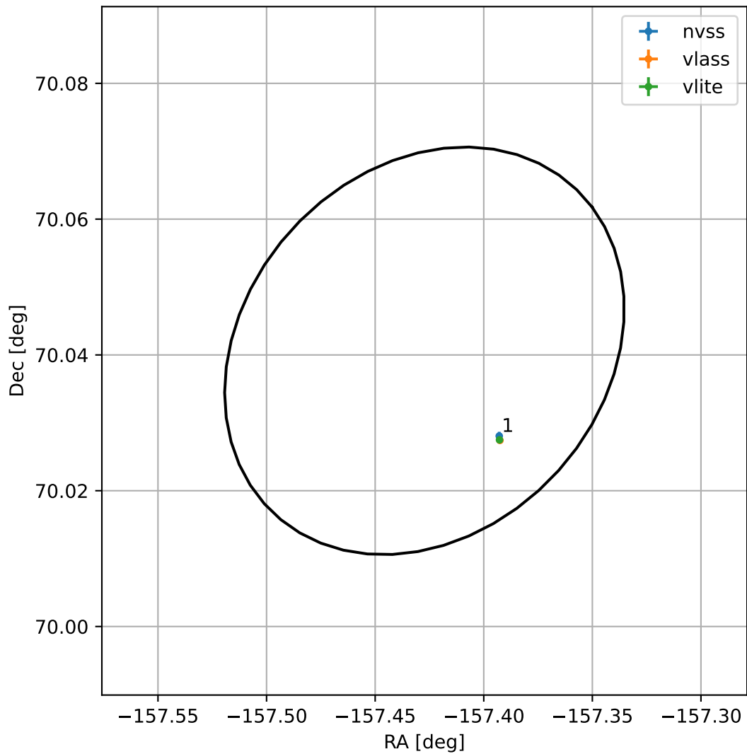
4FGL J1330.2+7002
