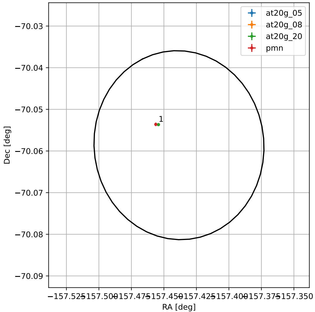
4FGL J1330.2-7003
