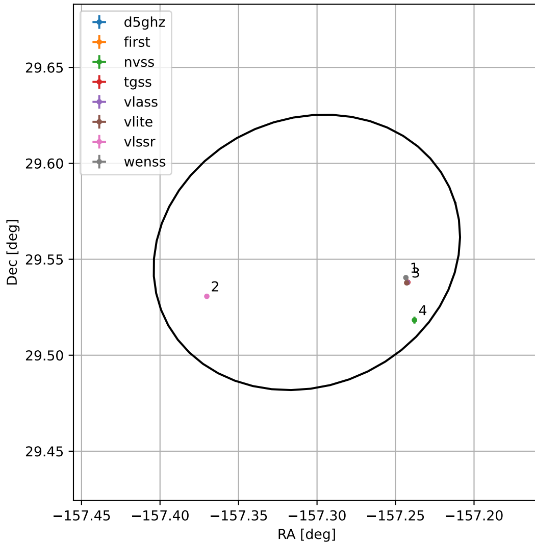
4FGL J1330.7+2933
